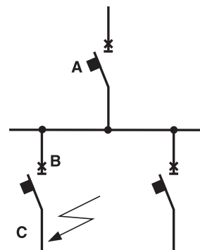
Circuit diagram with selective coordination of protections
