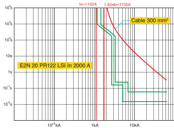
Time-Current Curve LLL
