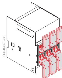
Front terminals
