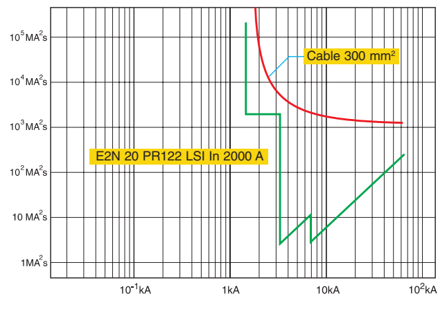
Specific let-through energy curve LLL
