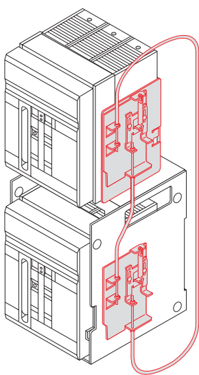
Vertical interlock
