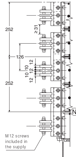
View A
