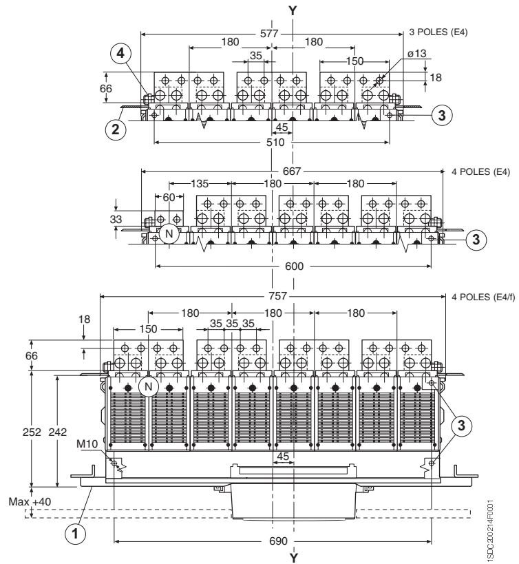
View A
