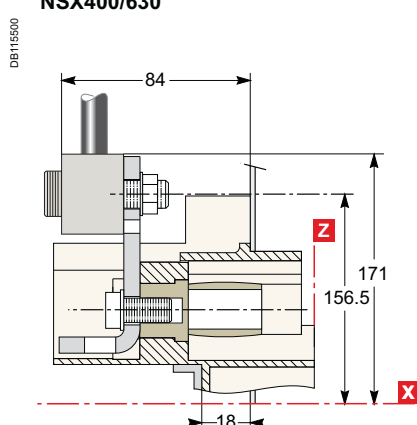
NSX400/630
