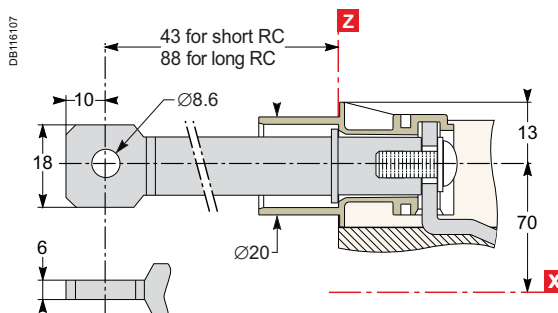
NSX400/630
