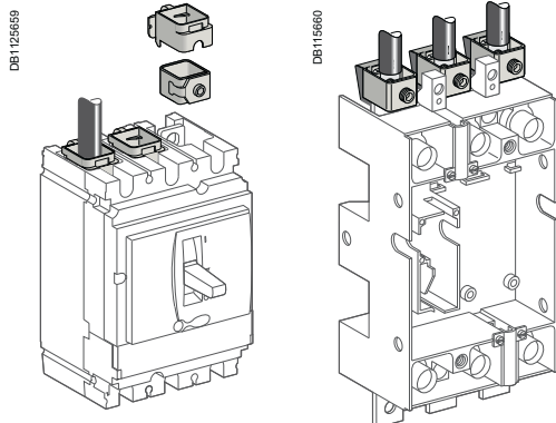
1-cable connector
