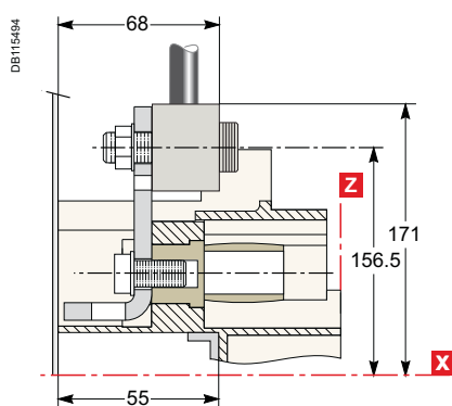
NSX400/630
