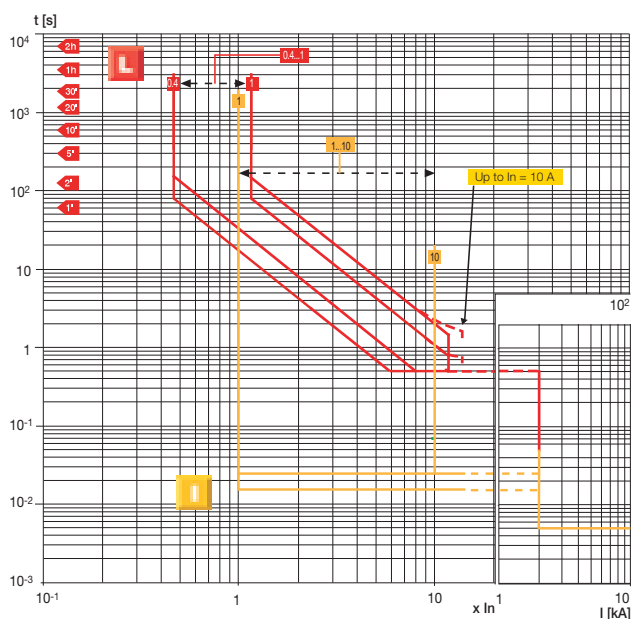
T2 160 – PR221GP
