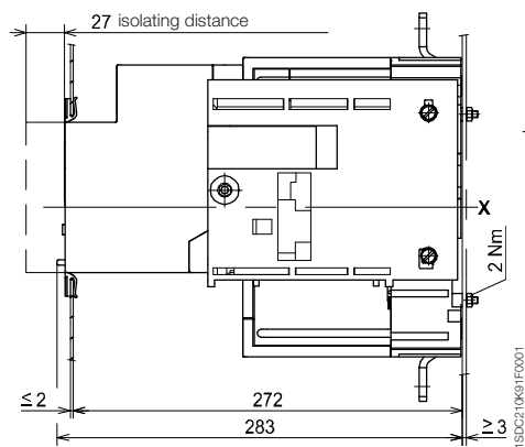
T5 (630 A)
