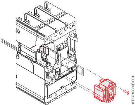
T4-T5-T6
