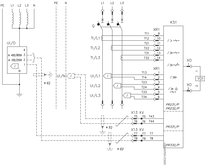
Three-pole circuit-breaker with PR231/P, PR232/P, PR331/P, PR332/P electronic trip unit
