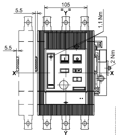
T5 (400 A)
